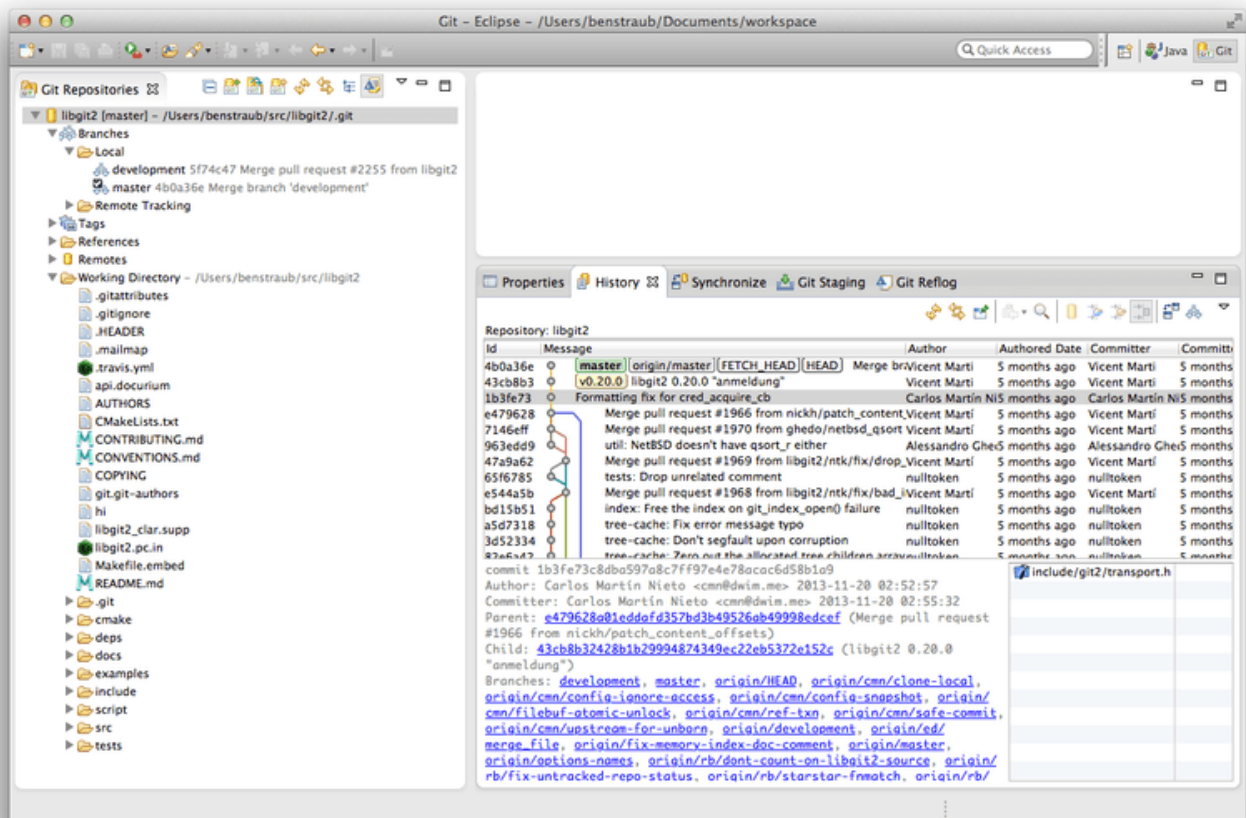
Figure 161. Eclipse's EGit environment.
