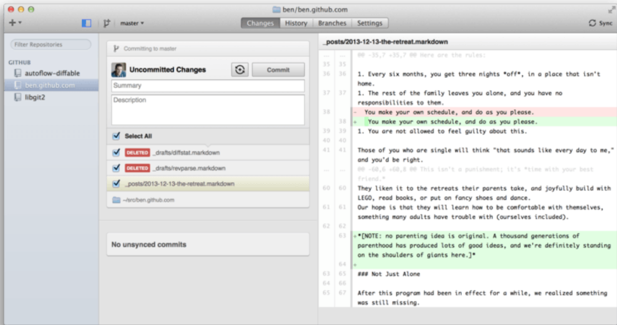
Figure 155. GitHub for macOS.
