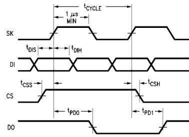
FIGURE 9. NM93C06A Timing
