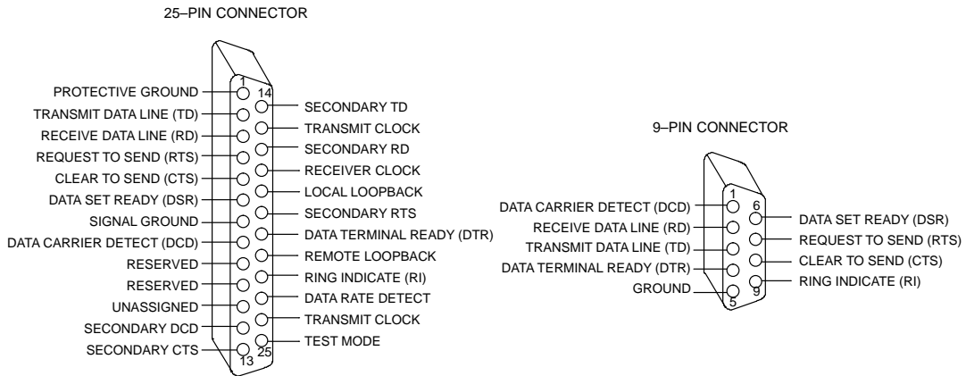
RS-232 CONNECTOR PIN ASSIGNMENTS Figure 2
