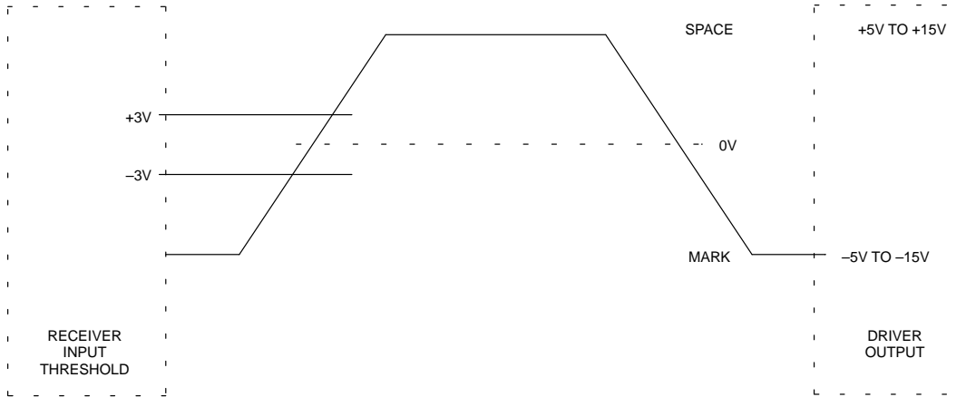
RS-232 LOGIC LEVEL SPECIFICATIONS Figure 1
