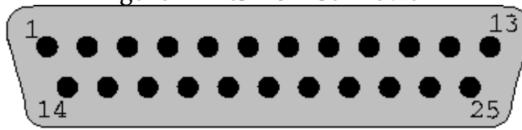
Figure 2 - RS-232 Connector
