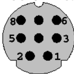
Figure 6 - SGI 8-Pin Connector
