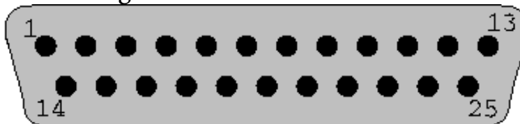
Figure 3 - RS-422 Connector
