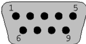
Figure 4 - RS-574 Connector
