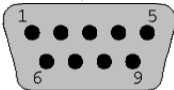
Figure 5 - SGI 9-Pin Connector
