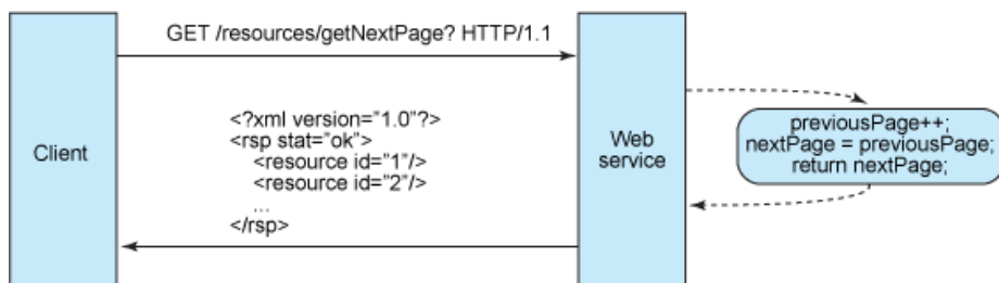
Figure 1. Stateful design
