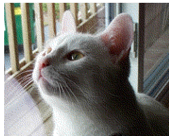
Cat at reduced depth with dithering
