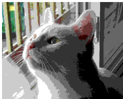
Cat at reduced depth without dithering
